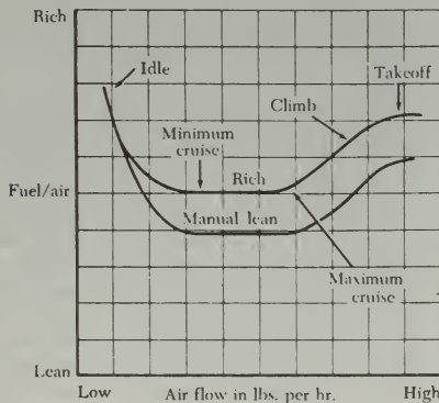
FIGURE 10-38. Typical fuel/air mixture curve for float-type carburetor.
